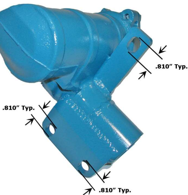
Pic1: Modified mounting holes
