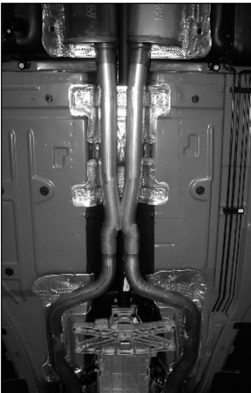
Cat-back Exhaust System Includes: X-pipe, Mufflers & Tailpipes.
