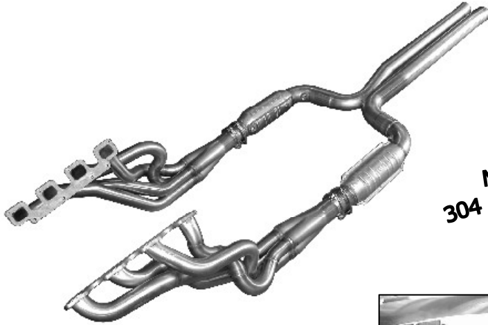
1-7/8" Headers with 3" collectors Includes: Gaskets & Hardware
